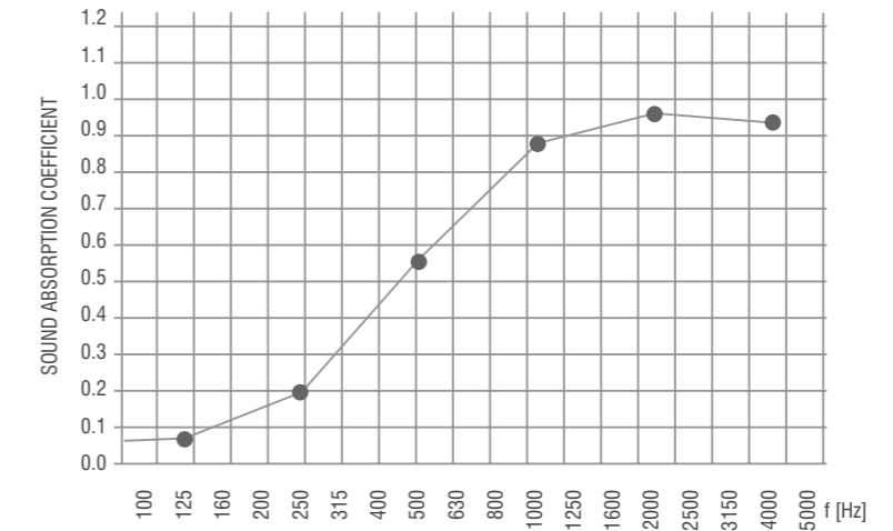
BUZZISKIN 3D ALFA SABINE TEST
